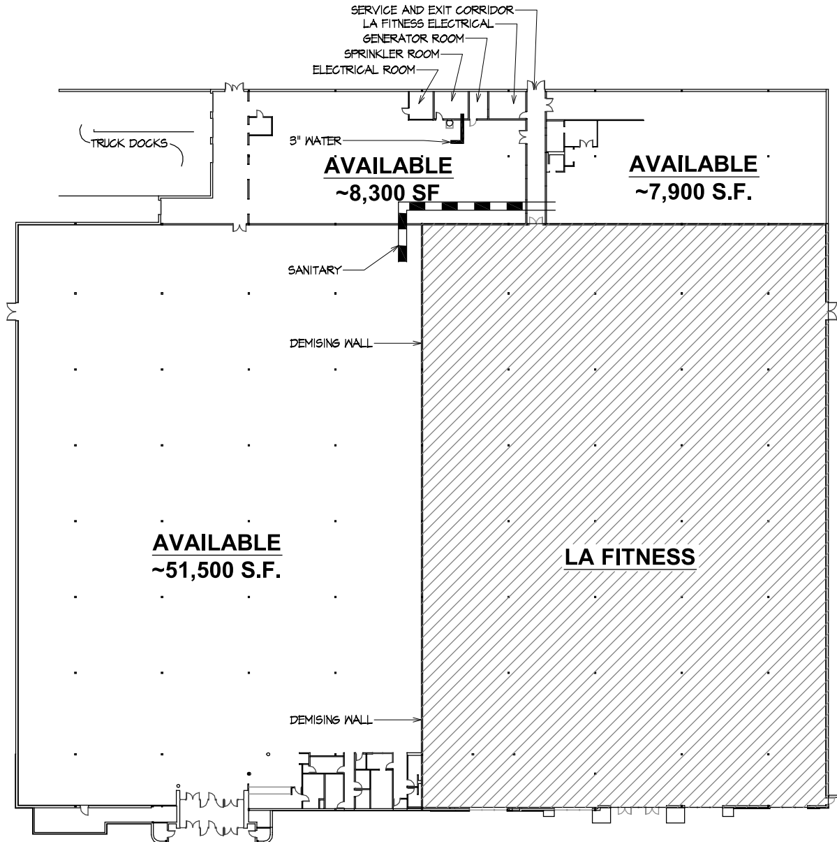
UTILITY PLAN
